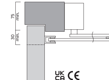
Fig.61 Transom mount push side
