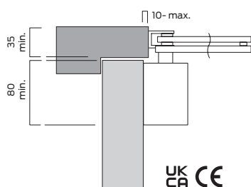
Fig.1 Door mount pull side
